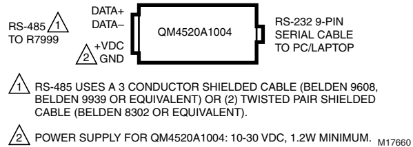
Fig. 4. QM4520A RS-485 to RS232 Converter.
